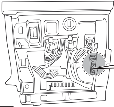
fuse holder
